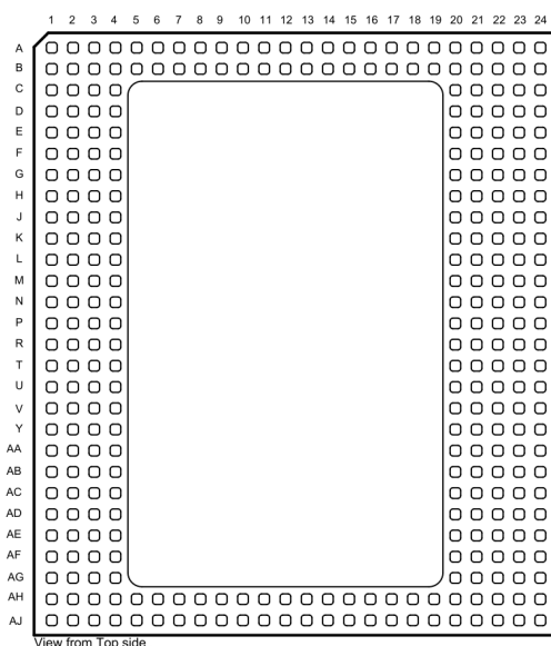
Figure 2: Grinn GenioSOM-510 pads (top view)
