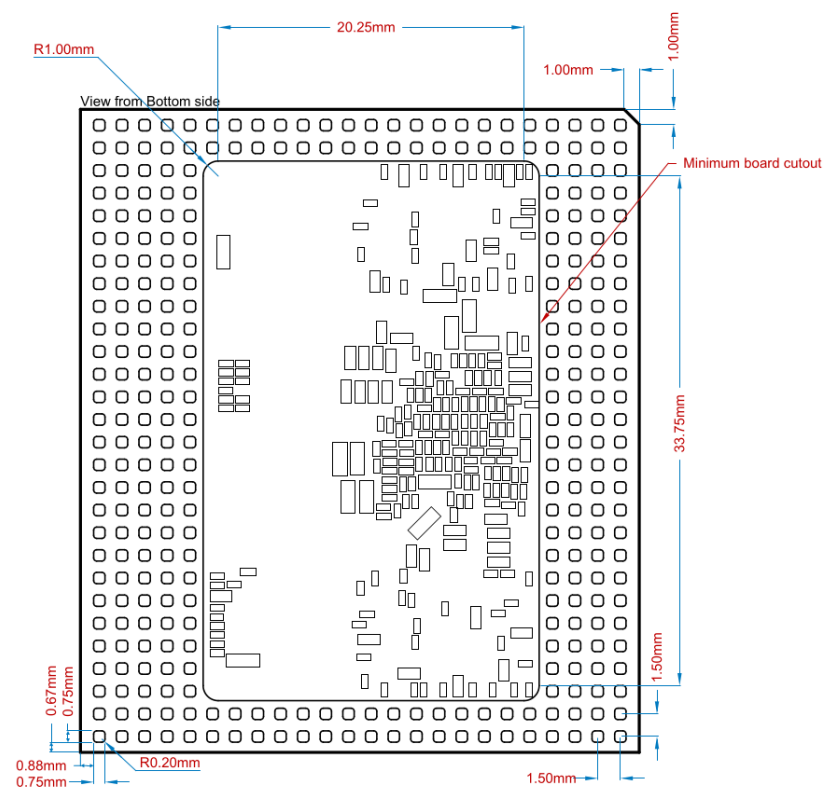
Figure 8: Grinn GenioSOM-510 bottom view dimensions
