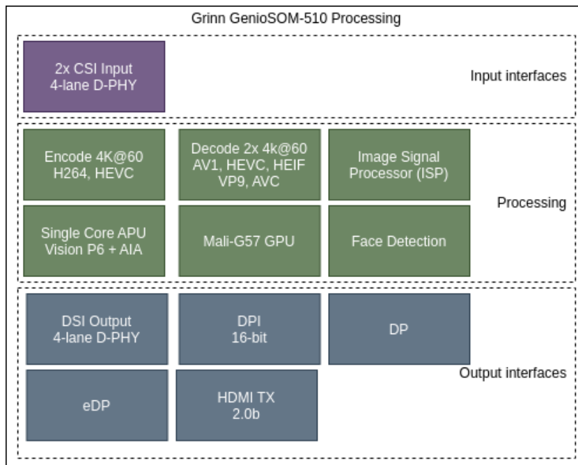
Figure 5: Grinn GenioSOM-510 video processing
