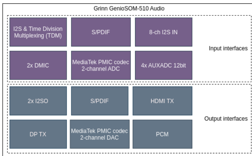
Figure 6: Grinn GenioSOM-510 audio interfaces
