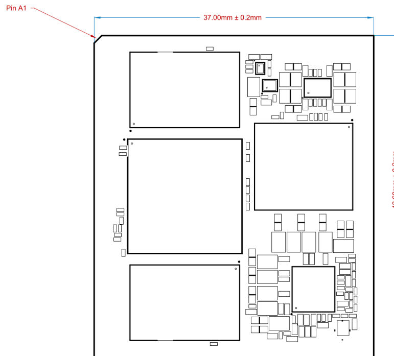
Figure 7: Grinn GenioSOM-510 top view dimensions
