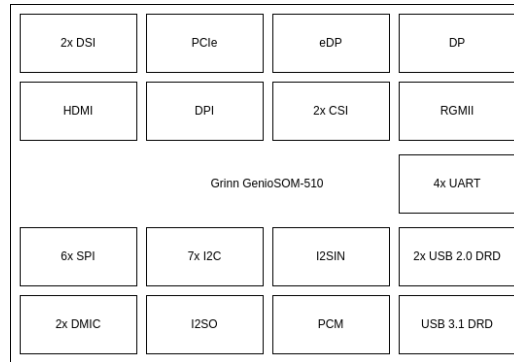
Figure 4: Grinn GenioSOM-510 interfaces overview
