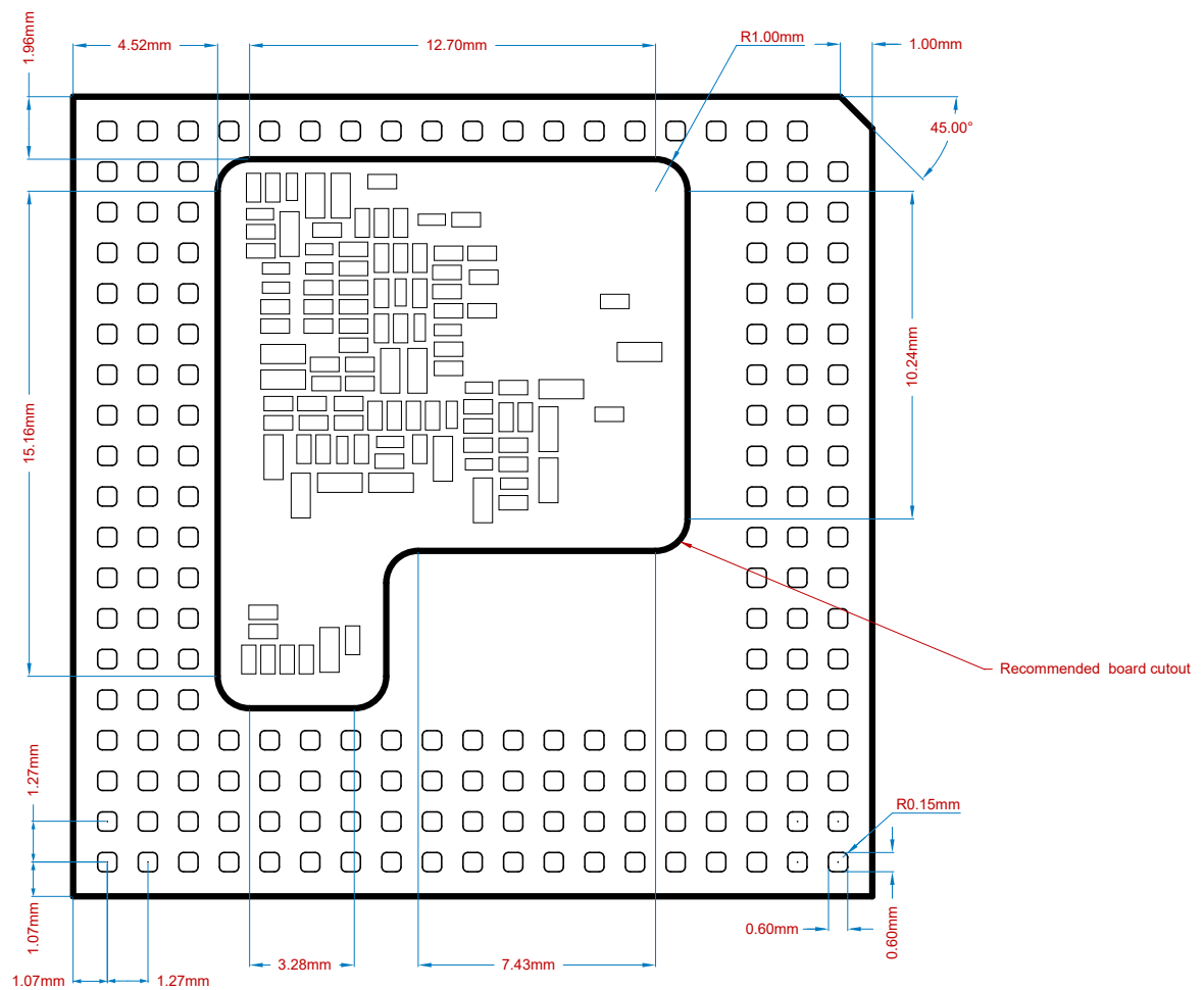
Fig. 5: Grinn AstraSOM-261x (View from Bottom side)
